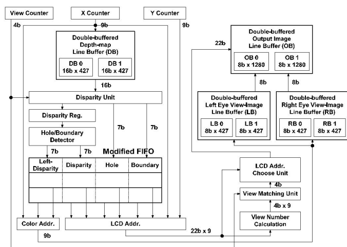
Figure 15.4.5: Block diagram of a sub-pixel unit.
