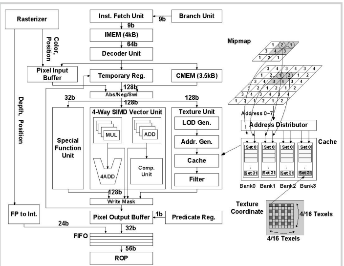
Figure 15.4.2: Block diagram of RE.
