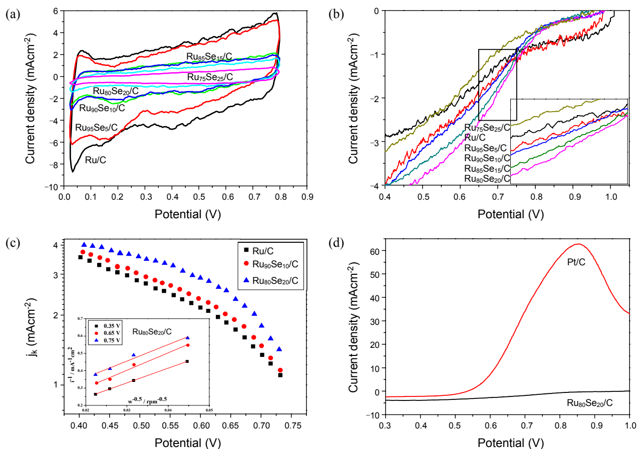
Figure 2. Electrochemical characterization; Cyclic voltammery results (a) and ORR results (b) for the Ru/C, Ru 95 Se 5 /C, Ru 90 Se 10 /C, Ru 85 Se 15 /C, Ru 80 Se 20 /C, and Ru 75 Se 25 /C catalysts. Tafel plots for the ORR of Ru/C, Ru 90 Se 10 /C, and Ru 80 Se 20 /C catalysts (c). Methanol tolerance results for the Ru 80 Se 20 /C catalyst (d).
