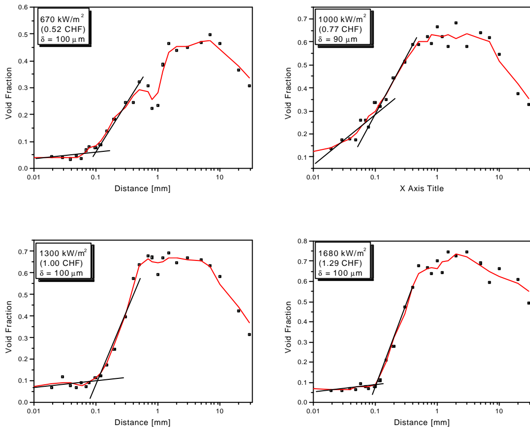
Fig. 7 Void fraction distribution (D=40 mm)
