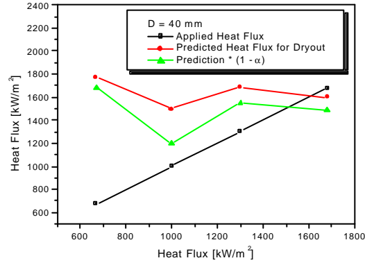
Fig. 10 CHF prediction using macroalayer thickness and bubble departure frequency
