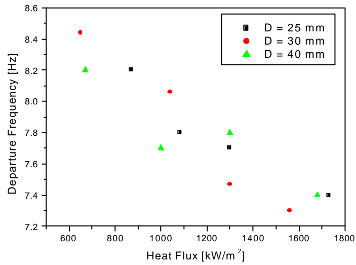
Fig. 9 Bubble departure frequency
