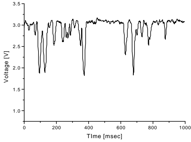
Fig. 3 Sample voltage signal from conduction probe
