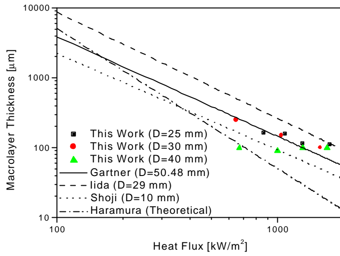
Fig. 8 Behavior of macrolayer thickness with heat flux
