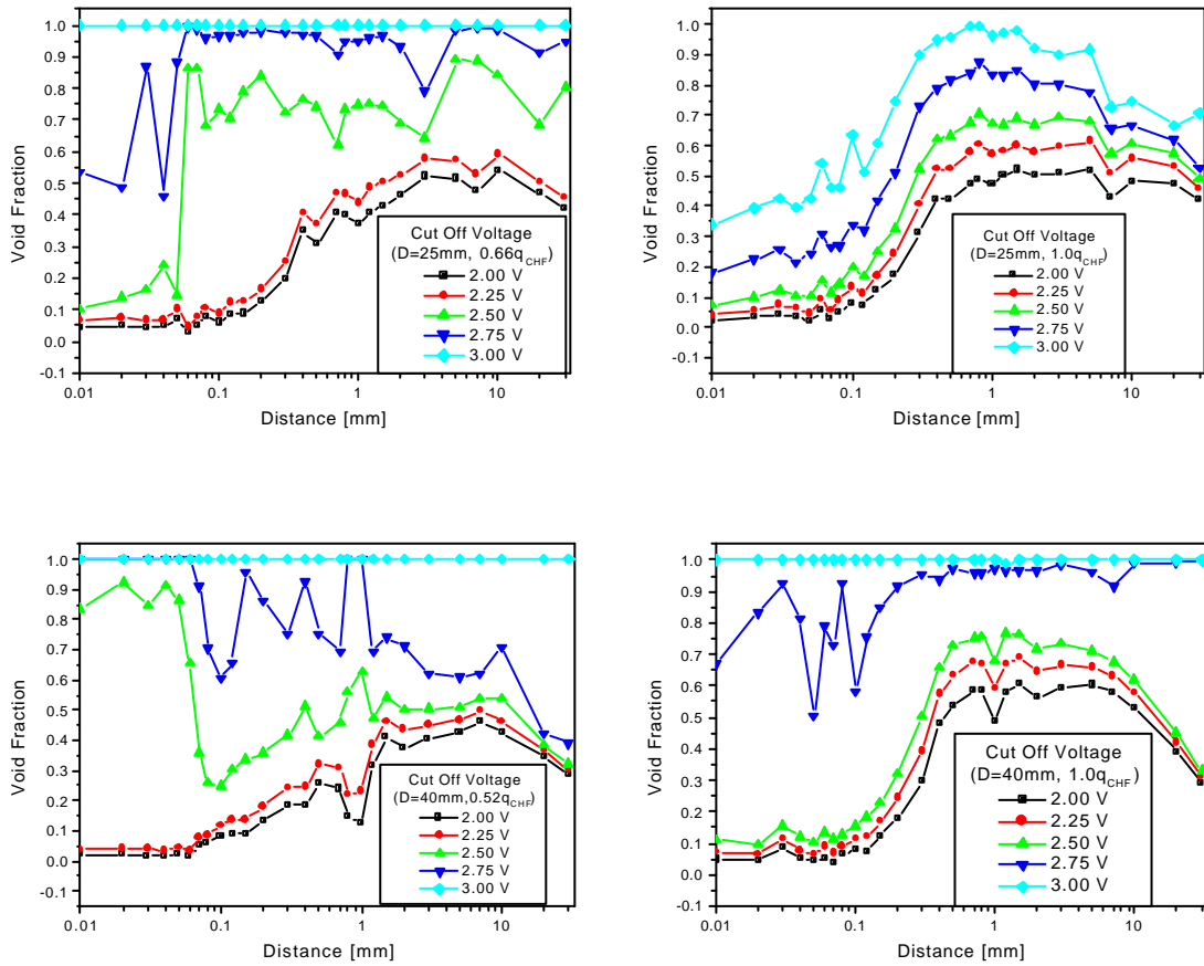
Fig. 4 Determination of cut-off voltage
