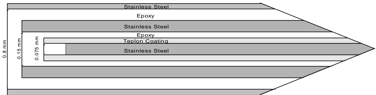
Fig. 2 Schematic diagram of conduction probe
