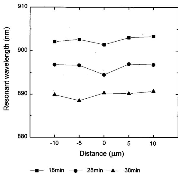
FIG. 4. Resonant wavelength variation over a mesa. The origin is taken at the center of the mesa. The resonant wavelength decreases with oxidation time.
