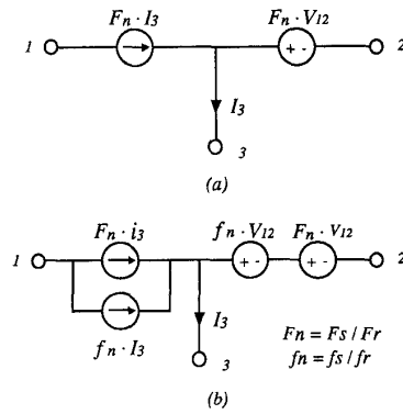
Fig. 15 DC and AC model of the CRS cell: (a) DC model, (b) AC model, capital letter: large signal, small letter: small signal.
