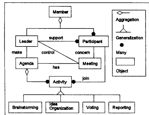
Fig. 1. Object model of meeting
