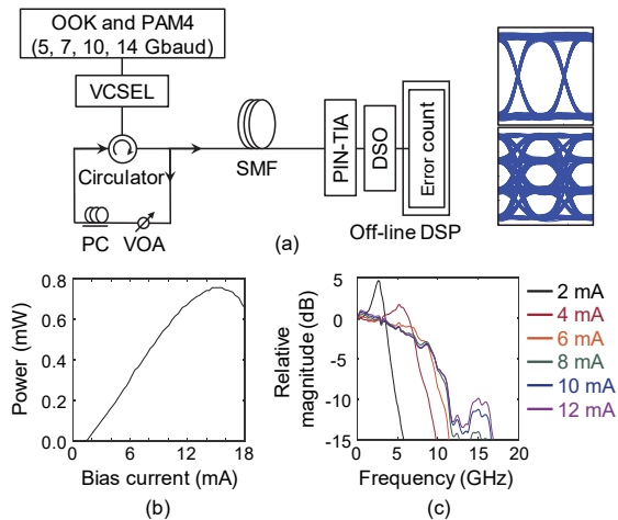
Fig. 1. (a) Experimental setup. (b) Measured L-I curve and (c) frequency response characteristics of the 1.55- \mu\text{m} VCSEL.
