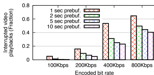
Figure 5: Fraction of interrupted playbacks across varying pre-buffering times and encoding rates.
