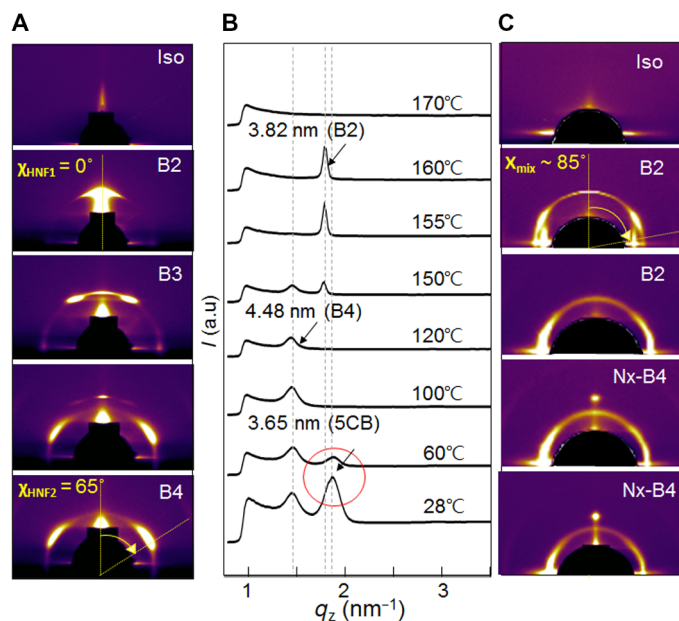
Fig. 2. In situ GIXD analysis tracing the thermal history of the 5CB-NOBOW 50:50 mixture in AAO upon cooling ( d_{\text{AAO}} = 60 nm). (A) Acquired 2D in situ GIXD images of neat NOBOW. (B) 1D vertical linecut for the 50 wt % mixture in the q range of 0.6 to 3.5 \text{nm}^{-1} , showing the evolution of the 2D diffraction peaks from the mixture and the 2D diffraction pattern. (C) In situ GIXD images of the 50:50 mixture of 5CB/NOBOW.
