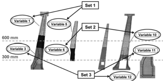
Fig. 6 Grouping of design variables with the height from the floor (Method 1)
