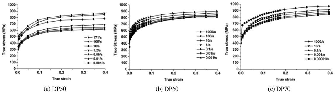
Fig. 3 Flow stress curves of DP steels with the variation of strain rates
