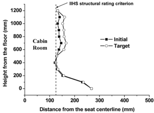
Fig. 5 Target shape for the thickness optimization
