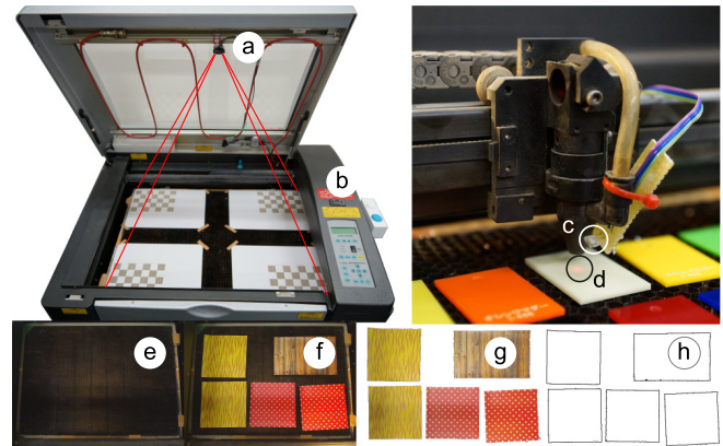
Figure 2. Top Left: an overlooking camera (a), mounted in the lid of a laser cutter for capturing materials, activated by a remote control attached to the side (b). Top right: a method for capturing that uses a photodiode (c) mounted on the toolhead of the laser cutter. The presence of material is detected by the reflection (d) of the sensing laser. Bottom row: a captured empty (e) and full table (f), the transformed and masked material (g), and the extracted edges (h).
