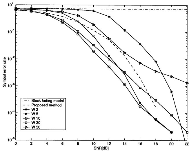
Fig. 6. SER. Single user with lowpass channel. Block fading assumption, RAKE with the proposed estimation, and RAKE with the decision-directed tracking with window size W .
