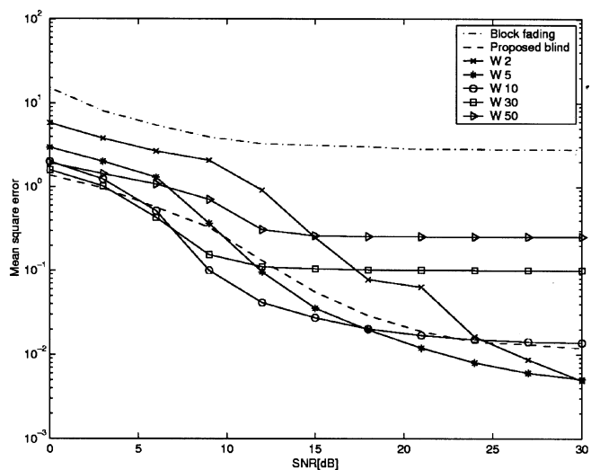
Fig. 5. MSE. Single user with lowpass channel. Block fading assumption, the proposed estimation, and the decision-directed tracking with window size W .
