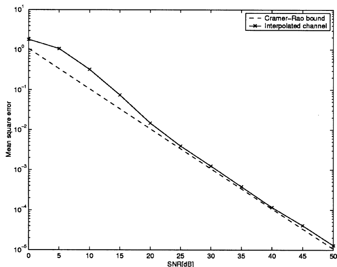
Fig. 3. MSE. Interpolated channel.
