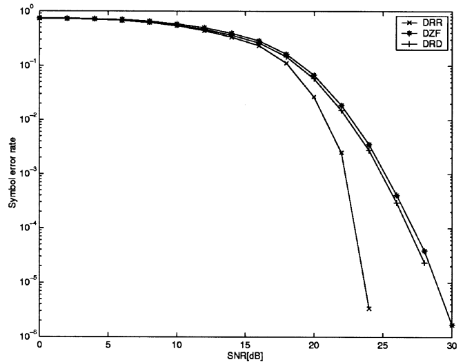
Fig. 7. BER. Four users with lowpass channel.
