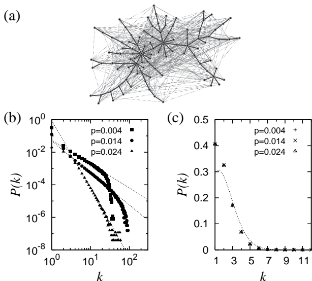
FIG. 1: (a) An illustration of topologies of the LST (solid line) and the original ER network (dotted line) with 100 vertices and p = 0.1 . (b) The degree distributions of the LSTs for various constructions of the ER networks with N = 4000 vertices and connection probability of edges p = 0.004, 0.014, 0.024 . The degree distributions are guided by the curve-fits (dotted lines) to P(k) \sim k^{-\gamma} with \gamma = 1.47, 1.97, 4.20 for p = 0.004, 0.014, 0.024 , respectively. (c) The degree distribution of the LST when the weights are randomly redistributed on the edges. The Poisson degree distribution with average degree 2 of trees (dotted line) is given for comparison. All data points are obtained from the averages over 256 network ensembles.
