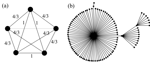
FIG. 4: (a) An example of the very dense network in which only one edges (dotted line) are eliminated from the fully connected network. The edge-BCs are given on the edges, which indicates that the edges of smaller degree vertices have more edge-BCs than the other edges. (b) Typical topology of the LST for very dense ER network. The structure is obtained from the ER network with N = 100 vertices and connection probability p = 0.95 .
