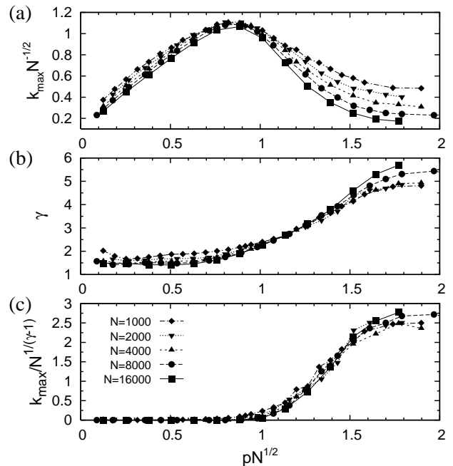
FIG. 3: The p dependence of (a) the average maximum degree k_{max} and (b) the power-law exponent \gamma in the degree distribution of the LST. In (c), the comparison of k_{max} with the natural cutoff N^{1/(\gamma-1)} is given. The data points are obtained from the averages over 256 ensembles.
