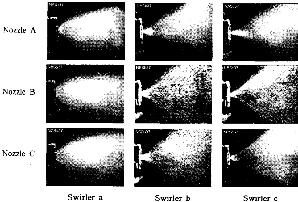
Fig. 7 Spray Visualization at AFR = 37
