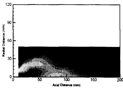
(e) Temperature at AFR = 37
