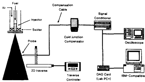
Fig. 3 Temperature measurement
