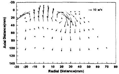
(a) Swirler a
