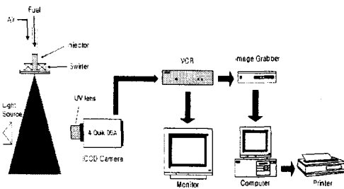
Fig. 4 Visualization setup
