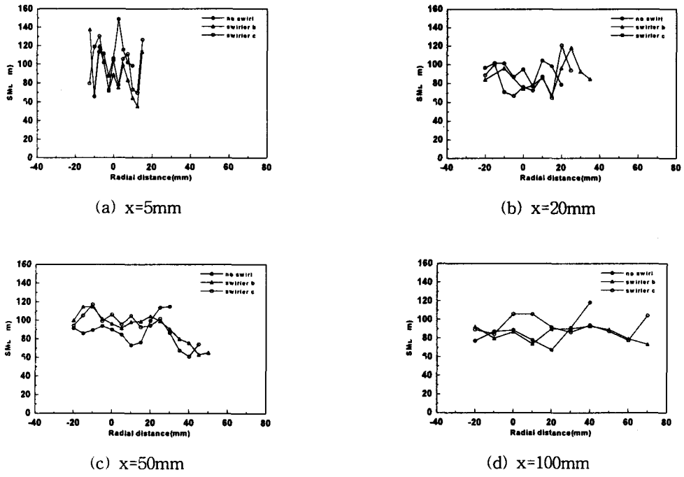
Fig. 6 SMD distribution of nozzle A (air=0.04kg/s, fuel=320cc/min)
