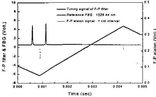
Fig. 3 Tuning signal of F-P filter and optical signal of the reference FBG and an F-P etalon.
