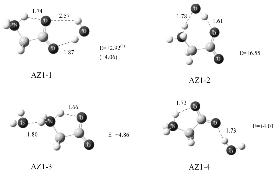
FIG. 3. Structures and relative energies (kcal/mol) of Gly-(H 2 O) 1 - anion complexes with zwitterionic Gly core. (a) Relative energy compared to global minimum energy structure AN1-1 with the canonical Gly core.
