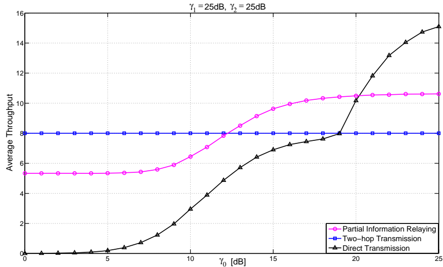
Fig. 4. Average throughput when \gamma_1 = 25 dB, \gamma_2 = 25 dB, and M = N = 4 .
