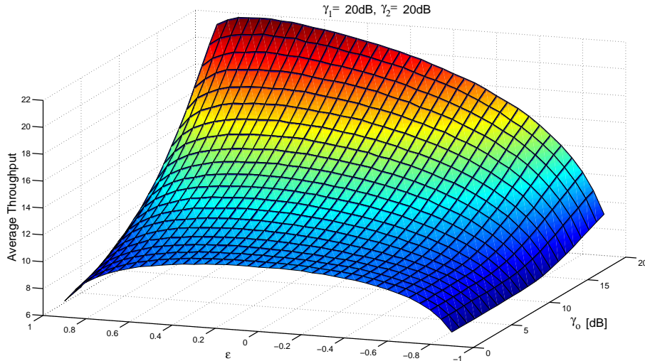
Fig. 3. Capacity (bits/symbol) versus \gamma_0 and \epsilon when \gamma_1 = 20 dB, \gamma_2 = 20 dB, and M = N = 4 .
