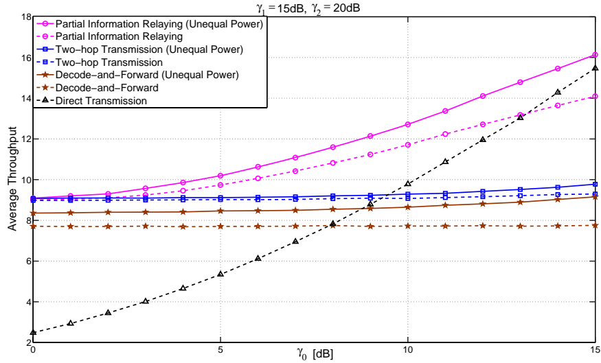
Fig. 1. Capacity (bits/symbol) when \gamma_1 = 15 dB, \gamma_2 = 20 dB, and M = N = 4 .
