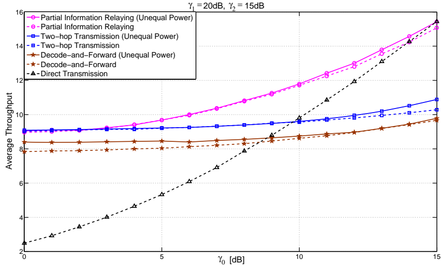
Fig. 2. Capacity (bits/symbol) when \gamma_1 = 20 dB, \gamma_2 = 15 dB, and M = N = 4 .
