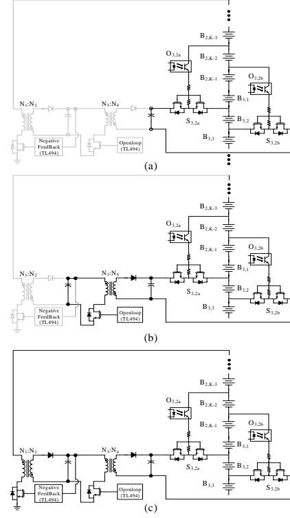
Fig. 2. Operational principles of the proposed circuit.
